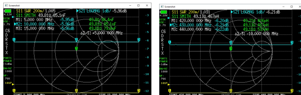
Attenuator board: 10 MHz and 430 MHz, nominal 6dB attenuation.
